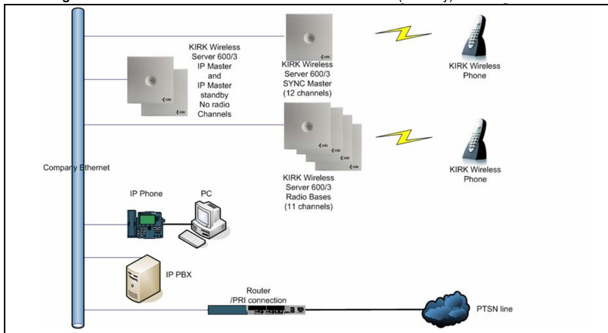
Figure 60 KWS600v3 Multi-cell installation with Alternative (Standby) Master
